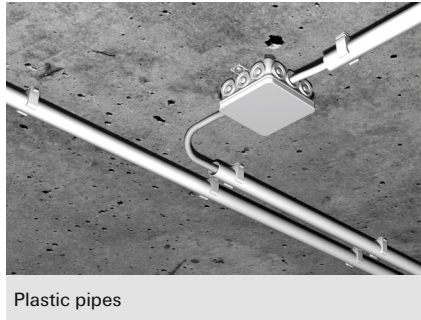
Flexible and rigid plastic insulation pipes
